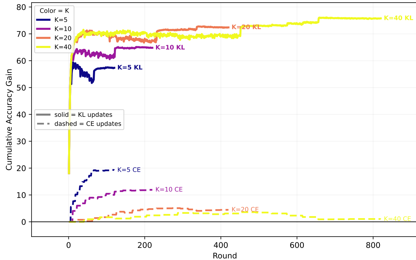
CE-pretrained teacher
