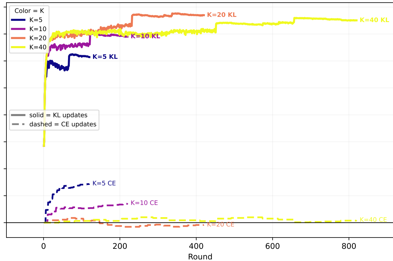
KL-self-distilled teacher
